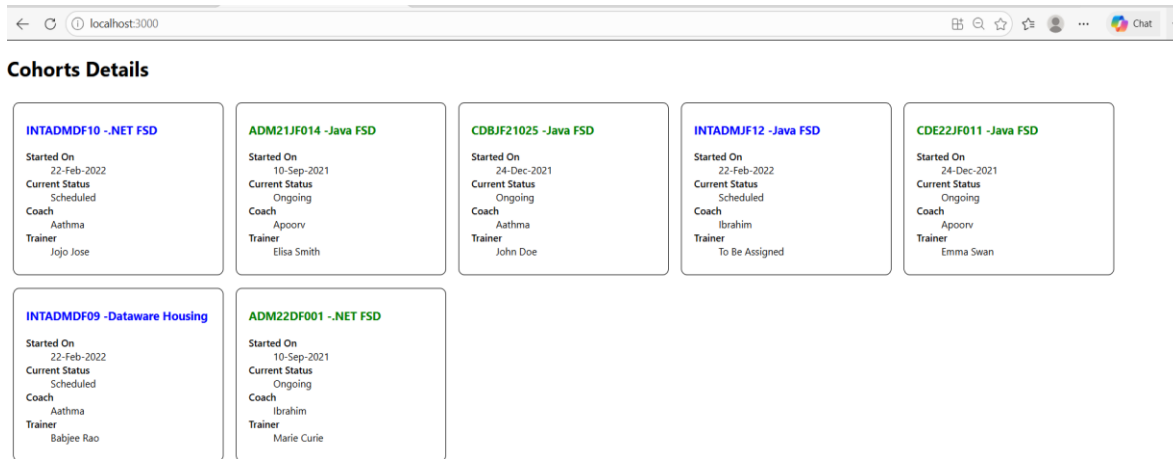
Figure 2: Browser Output
